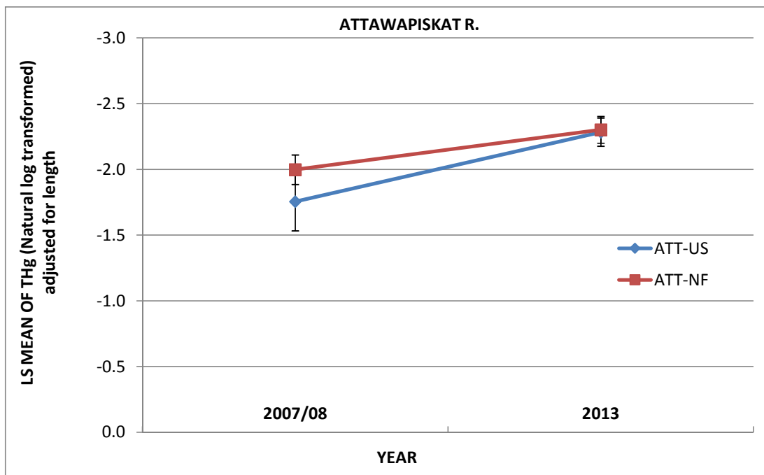
FIGURE 11: PLOT OF LS MEANS OF TRANSFORMED TOTAL MERCURY ADJUSTED FOR LENGTH LAKE WHITEFISH YEAR AND SITE COMPARISONS
