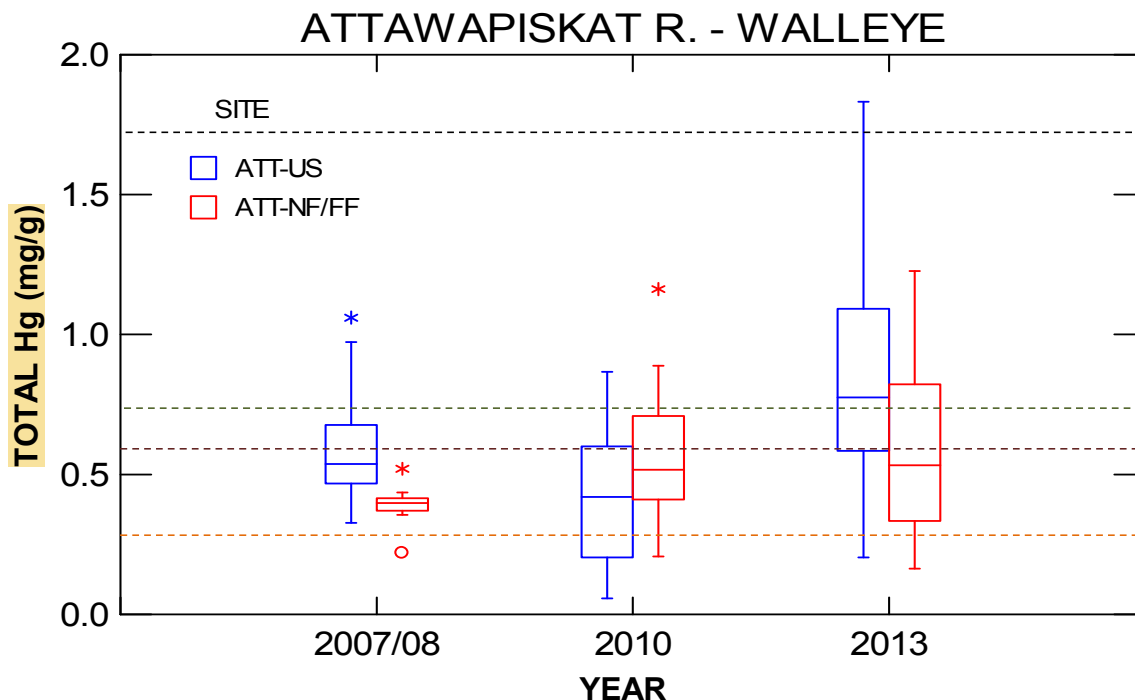
FIGURE 14: BOX PLOT SUMMARY OF TOTAL MERCURY CONCENTRATIONS FOR WALLEYE YEAR AND SITE COMPARISONS
