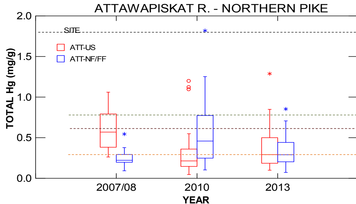
FIGURE 12: BOX PLOT SUMMARY OF TOTAL MERCURY CONCENTRATIONS FOR NORTHERN PIKE YEAR AND SITE COMPARISONS
